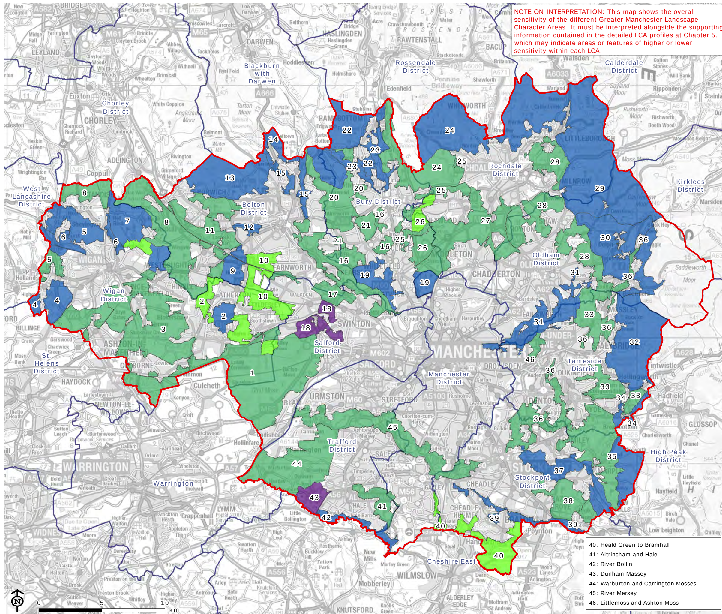
Figure 4.3: Overall Landscape Sensitivity Assessment results for residential development / related transport infrastructure
